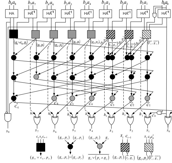
Fig. 2. Mod-257 TPP adder (Fig. 3 of [1], with outputs labeled s_i instead of r_i ).
