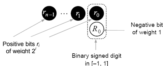
Fig. 5. Signed-LSB representation of \text{mod}-(2^n + 1) residues.
