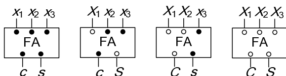
Fig. 6. The four functionalities of the same full-adder (FA) cell, with posibit and negabit inputs/outputs.
