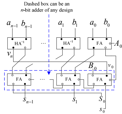
Fig. 9. Signed-LSB mod- (2^n - 1) addition process and its circuit realization.
