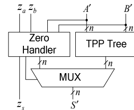
Fig. 4. Complete diminished-1 mod- (2^n + 1) adder with zero handler.
