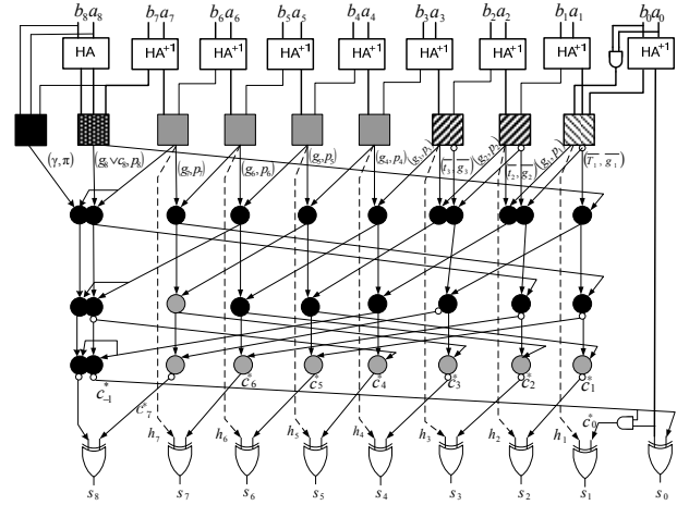
Fig. 3. The corrected mod-257 TPP adder.
