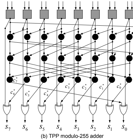
Fig. 1. Previously proposed designs for fast mod- (2^8 - 1) addition [2].
