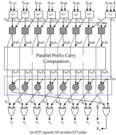
(a) RPP signed-LSB modulo-257 adder
