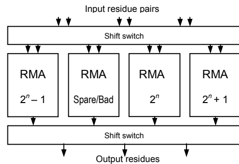
Fig. 11. Fault-tolerant RNS processor using reconfigurable mod- (2^n - 1)/2^n/(2^n + 1) adders.
